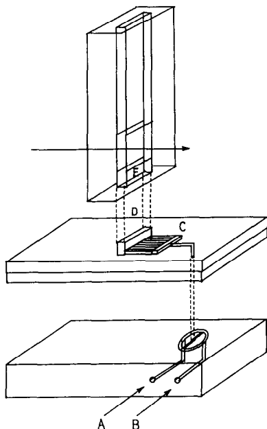
Fig.1. Diagrammatic representation of the modified slit-type mixer. Two solutions from inlets A and B are mixed in a double two-jet mixing part, divided into 8 flow lines at C and then expelled through a slit D (1 × 8 mm) to enter a flat observation cell E with laminar flow (see fig.2 of [4] for comparison).
